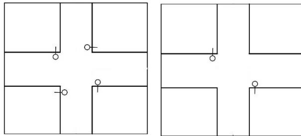
Figure 13 Modeled Luminaire Layouts for Rural Conventional Four-Leg Intersections
