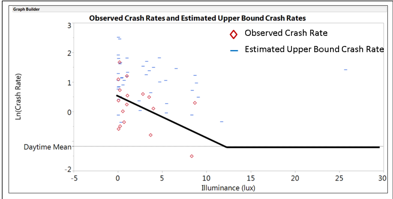
Figure 12 Observed Effect of Illumination Level on Total Crash Rates at Rural Intersections
